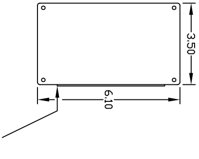
AE26-XXX (AE25, AE26 AVAILABLE IN ENCLOSURE SHOWN)
