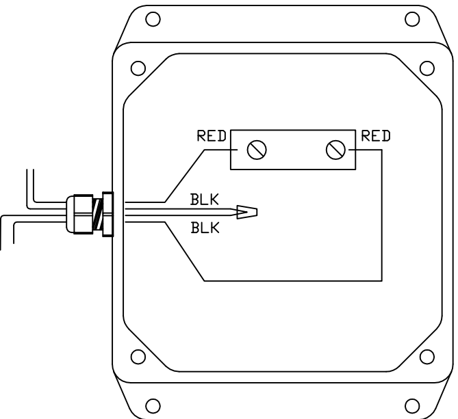
WIRING DETAILS
